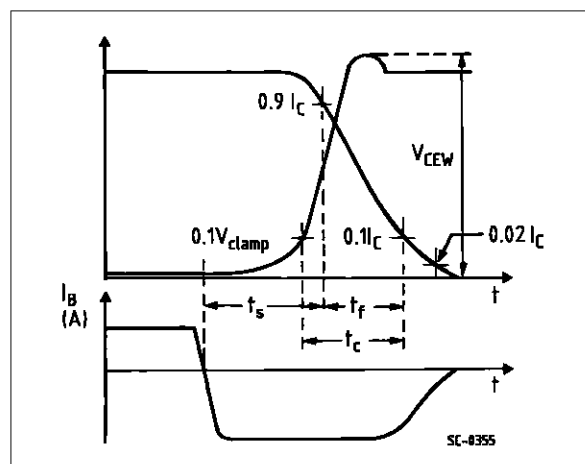
(2) Non-inductive load
