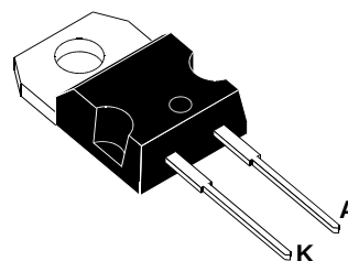
TO220AC (Plastic)
