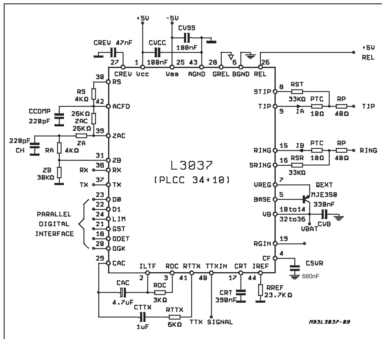
Figure 6: Test Circuit
