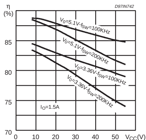
Figure 14. Efficiency vs. V_{CC} .
