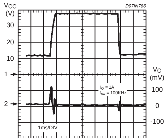
Figure 19. Line transient.
