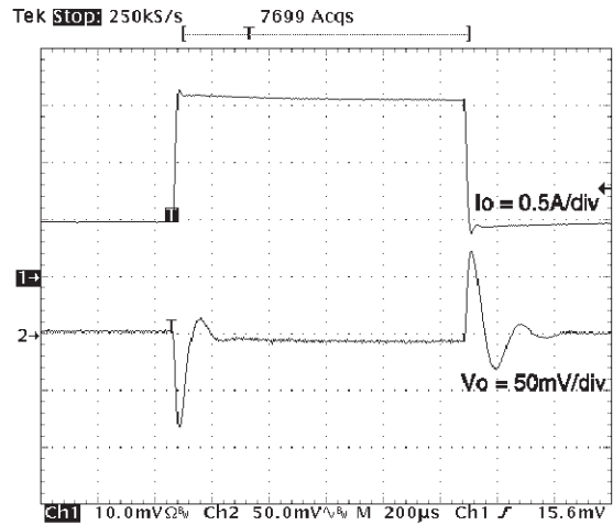
Figure 21. Load transient.
