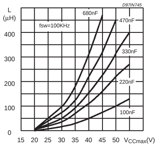
Figure 23. Soft start capacitor selection Vs inductor and Vccmax.
