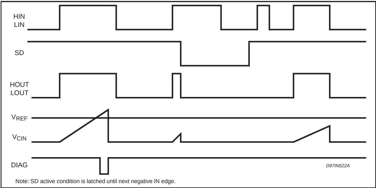
Figure 1. Timing Waveforms
