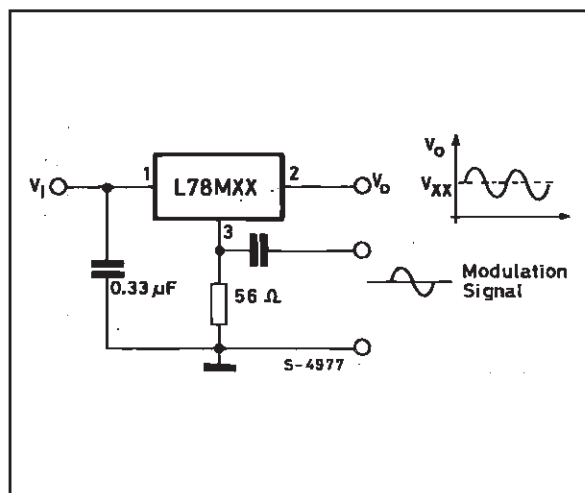
Figure 23 : Power AM Modulator (unity voltage gain, I_o \leq 0.5 ).
