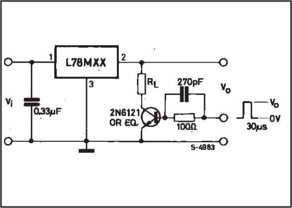
Figure 2 : Load Regulation.
