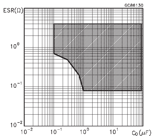
Figure 17 : Stability
