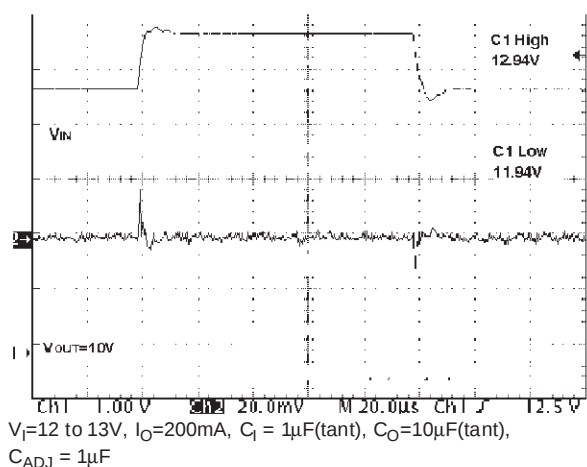
Figure 18 : Line Transient
