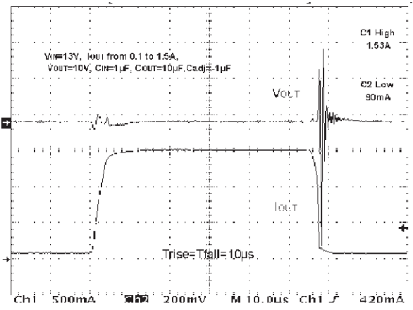
Load Transient
