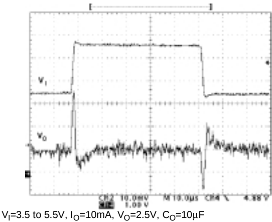
Figure 19: Line Transient
