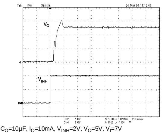
Figure 21: Start-Up Time 10mA
