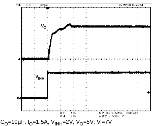
Figure 22: Start-Up Time 1.5A
