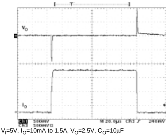
Figure 20: Load Transient
