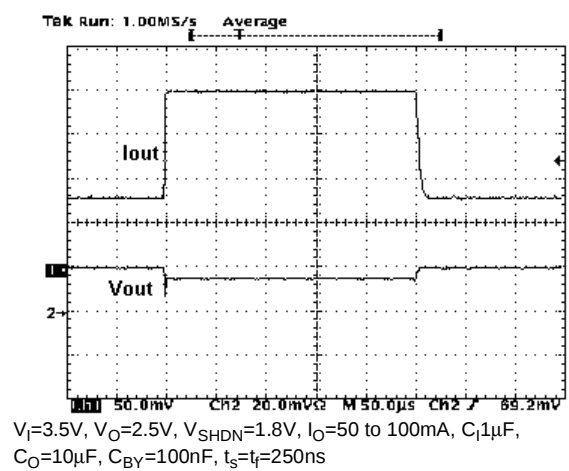
Figure 28 : Load Transient
