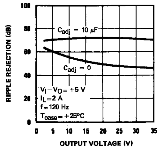
RIPPLE REJECTION
