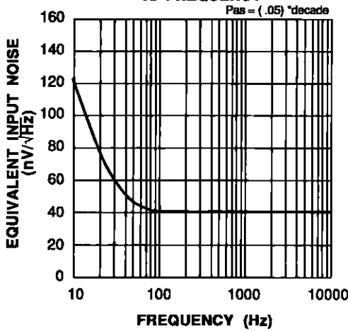
EQUIVALENT INPUT NOISE vs FREQUENCY
