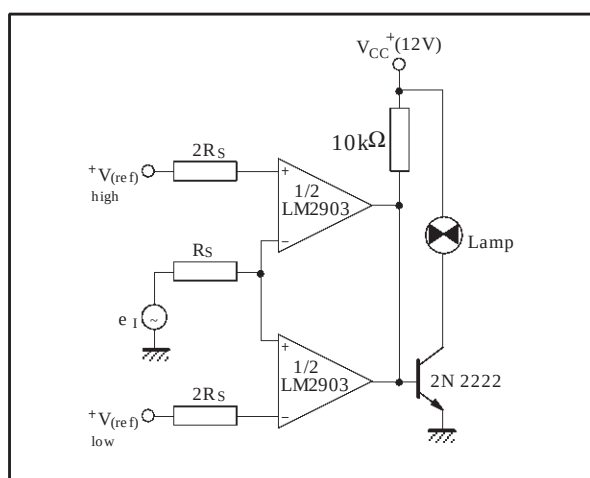
LIMIT COMPARATOR
