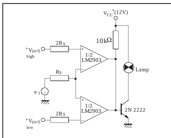
LIMIT COMPARATOR
