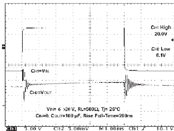
Line Transient
