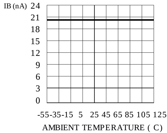
INPUT BIAS CURRENT versus AMBIENT TEMPERATURE
