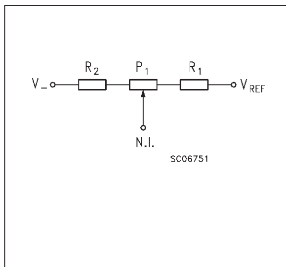
Figure 23 : Shunt Regulator.
