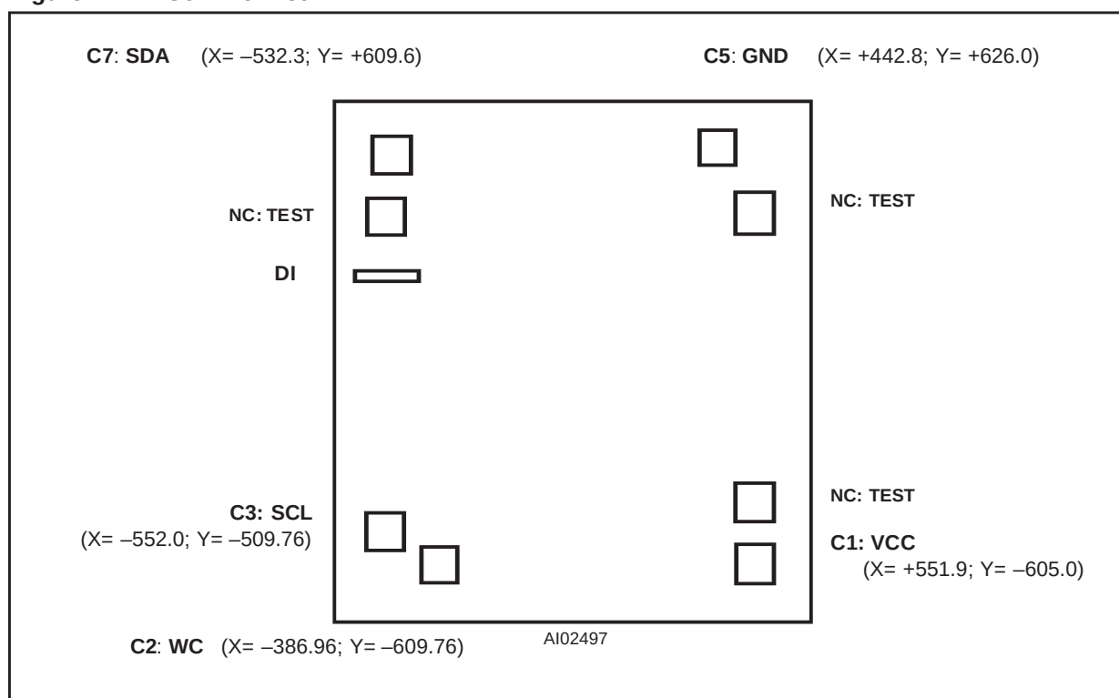
Figure 1. M14C04 Die Plot
