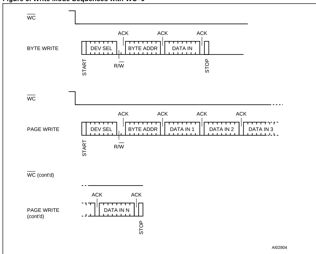
Figure 6. Write Mode Sequences with \overline{WC}=0
