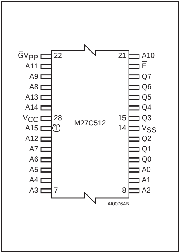
Figure 2C. TSOP Connections
