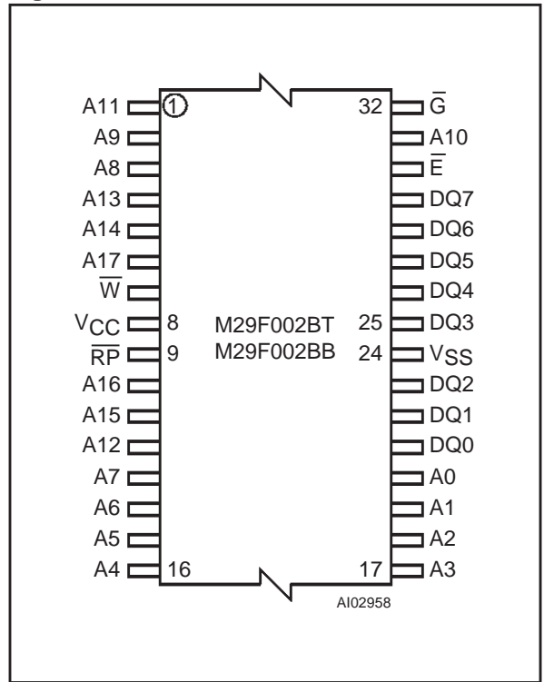
Figure 3. TSOP Connections
