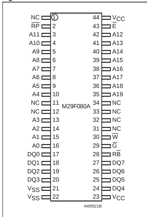
Figure 3. SO Connections
