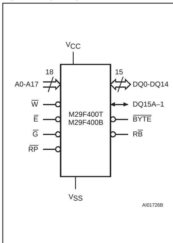
Figure 1. Logic Diagram
