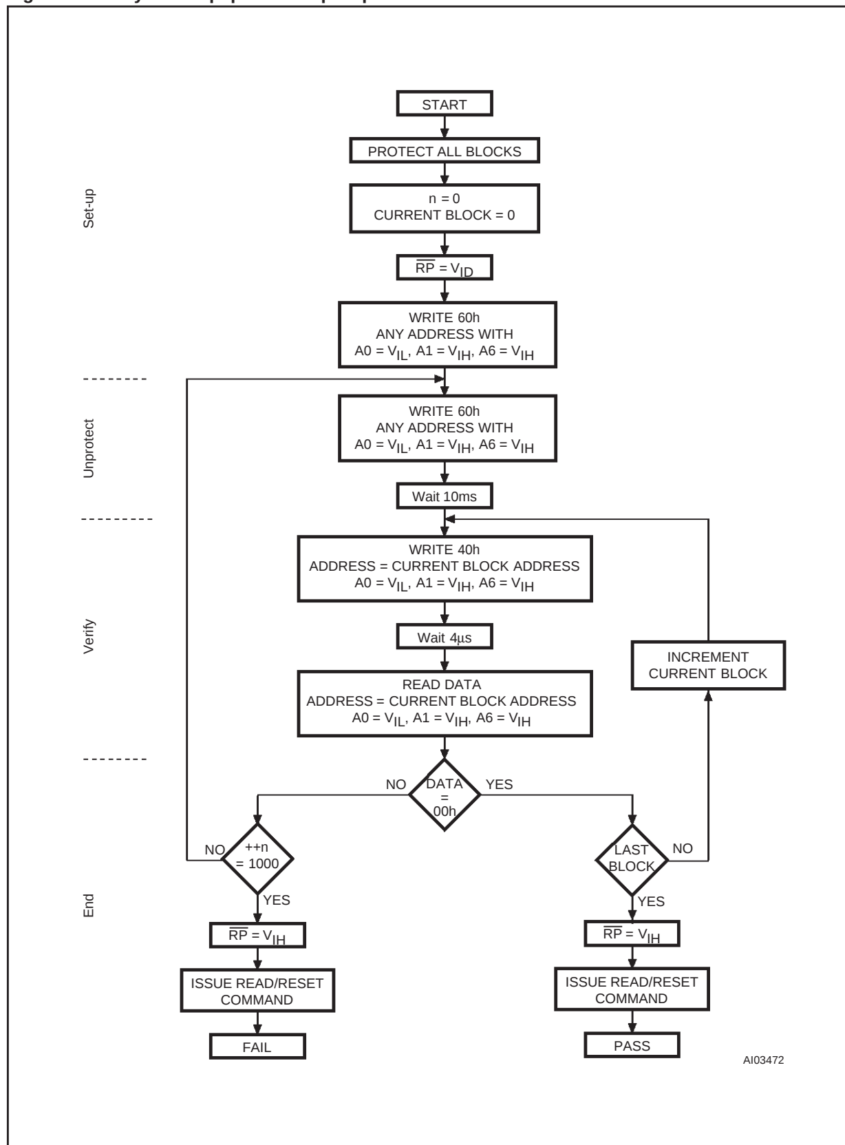
Figure 18. In-System Equipment Chip Unprotect Flowchart
