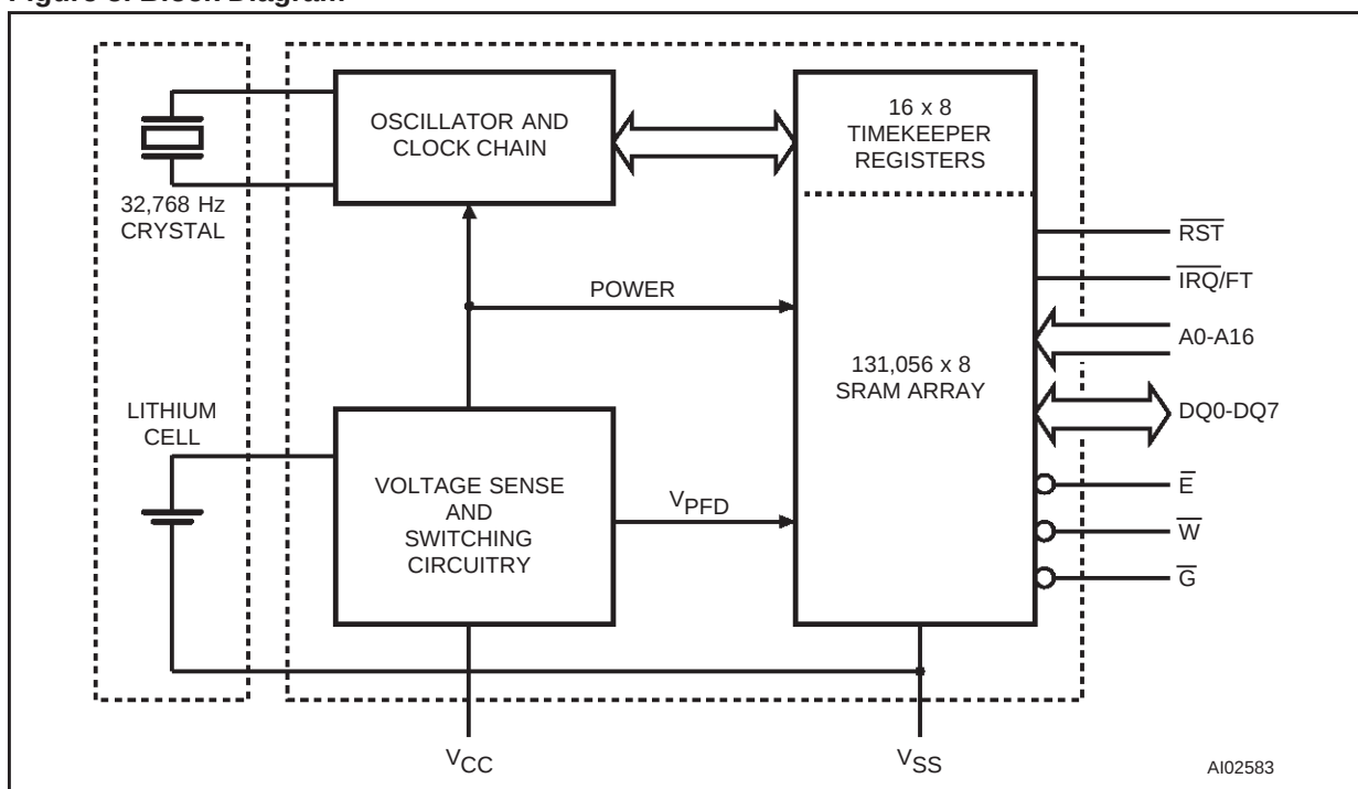
Figure 5. Block Diagram
