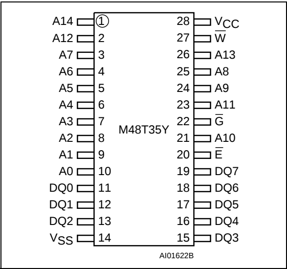
Figure 5. SOIC Connections
