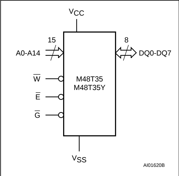
Figure 3. Logic Diagram
