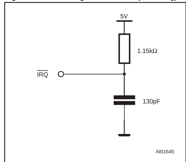
Figure 8. AC Testing Load Circuit (with \overline{\text{IRQ}} )
