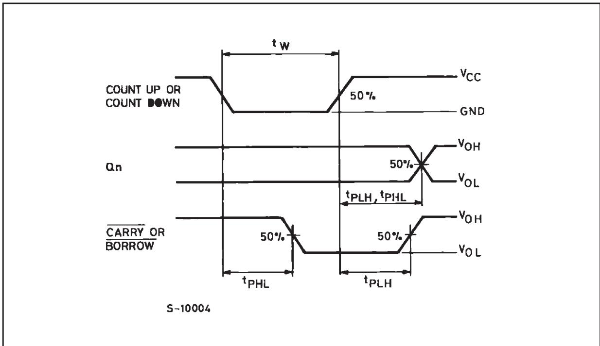
WAVEFORM 1 : PROPAGATION DELAY TIME, MINIMUM PULSE WIDTH (COUNT UP AND DOWN) ( f=1\text{MHz} ; 50% duty cycle)
