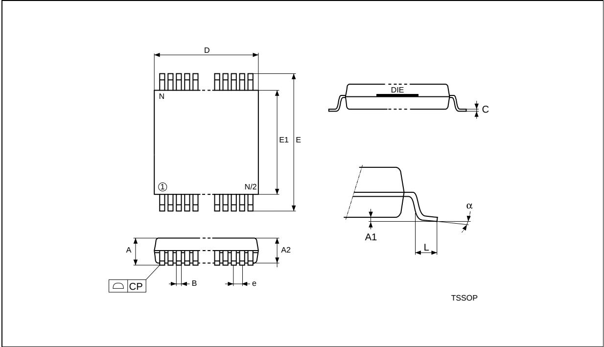
Figure 18. TSSOP14 (DL)
