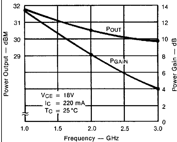
TYPICAL POWER OUTPUT &amp; GAIN @ 1dB COMPRESSION POINT vs FREQUENCY
