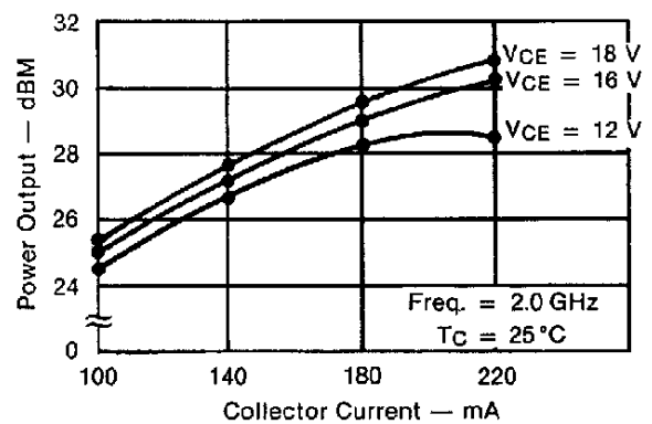
TYPICAL POWER OUTPUT &amp; GAIN @ 1dB COMPRESSION POINT vs COLLECTOR CURRENT
