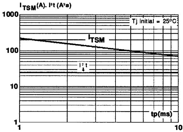
Fig.7 : Non repetitive surge peak on-state current for a sinusoidal pulse with width : t_p \leq 10\text{ms} , and corresponding value of I^2t .
