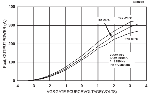
Output Power vs Gate Voltage
