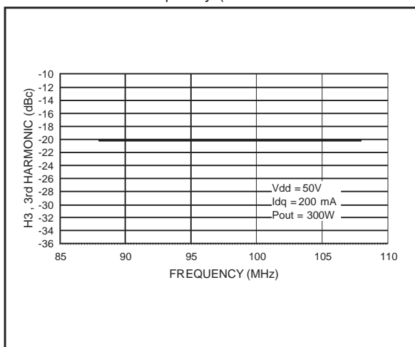
3rd Harmonic vs. Frequency (88 - 108 MHz)
