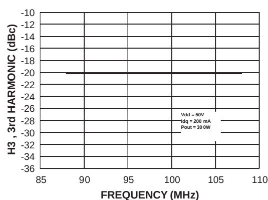
3rd Harmonic vs Frequency (88 - 108)
