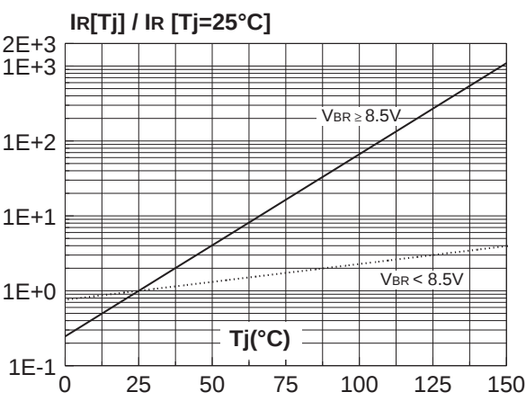
Fig 8: Relative variation of leakage current versus junction temperature.
