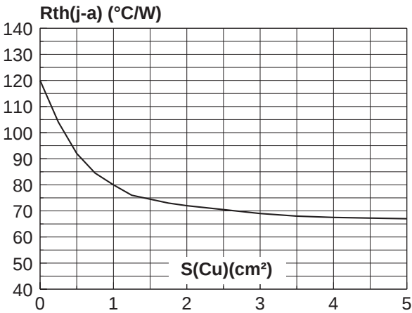
Fig 7: Thermal resistance junction to ambient versus copper surface under each lead (printed circuit board FR4 e(Cu)=35μm).
