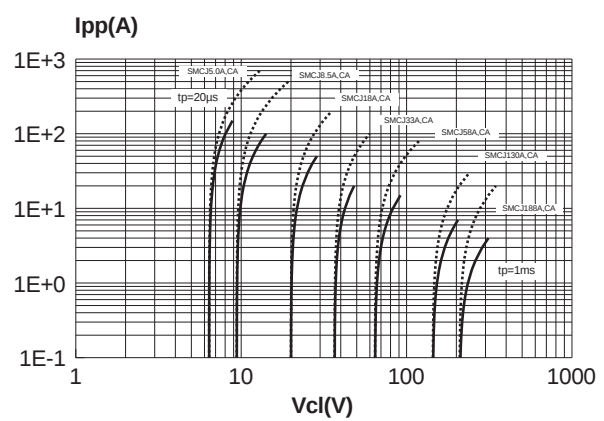
Fig. 4: Clamping voltage versus peak pulse current ( T_j initial= 25^\circ\text{C} ). Exponential waveform t_p=20\mu s & t_p=1ms .
