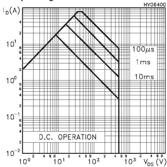
Safe Operating Area For TO-220/ I PAK /D PAK
