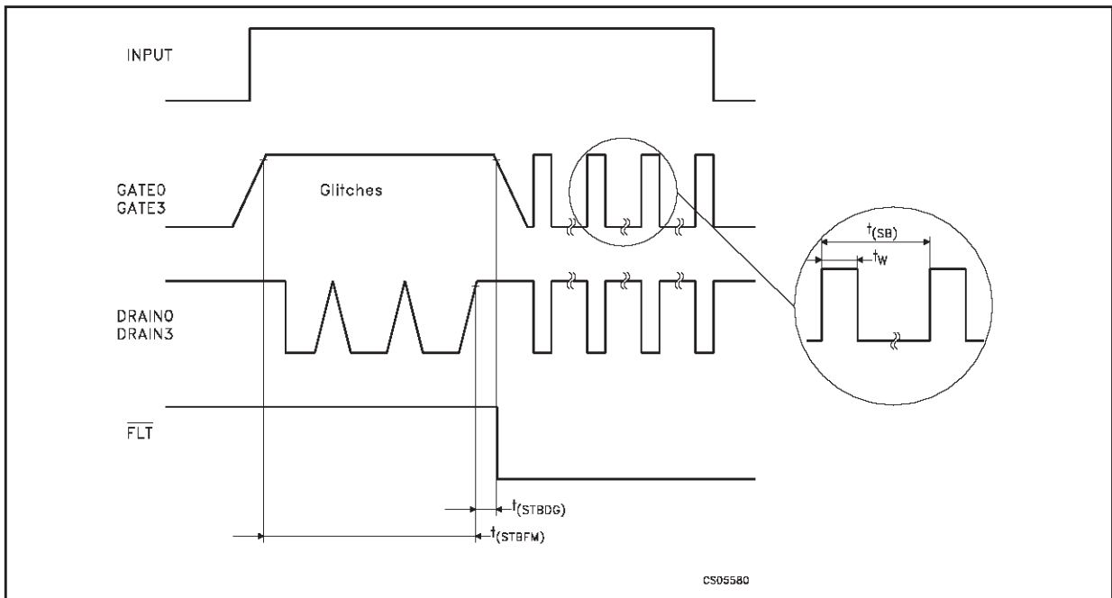
Figure 16 : Shorted Load Condition (Deglitch Time)
