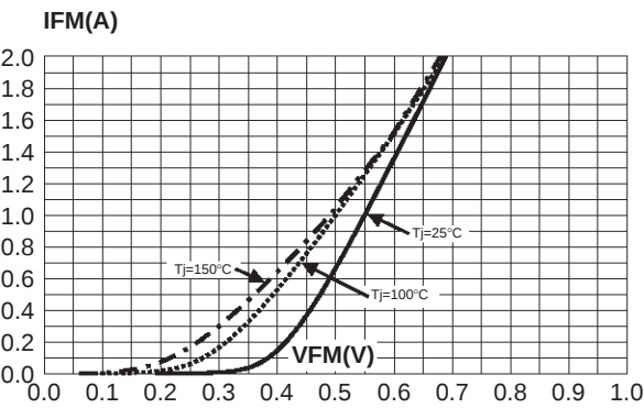
Fig. 8-2: Forward voltage drop versus forward current (low level, maximum values).
