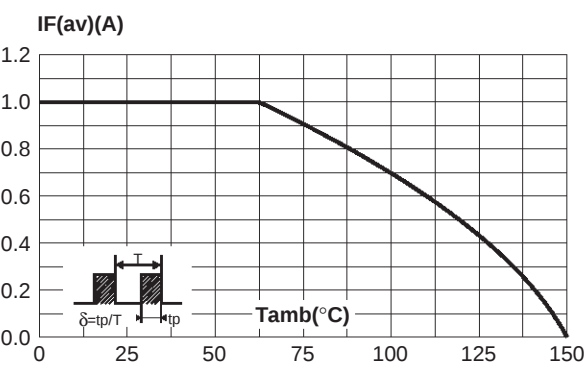
Fig. 2: Average forward current versus ambient temperature ( \delta=1 ).
