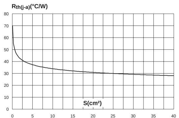
Fig. 9: Thermal resistance junction to ambient versus copper surface under tab (Epoxy printed circuit board, Cu = 35 \mu m ) (STPS20150CG only).
