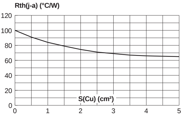
Fig. 9: Thermal resistance junction to ambient versus copper surface under each lead (Epoxy printed circuit board FR4, copper thickness: 35μm) (SMB).
