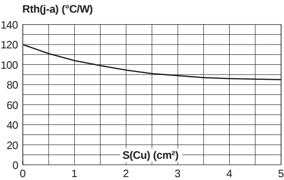
Fig. 10: Thermal resistance junction to ambient versus copper surface under each lead (Epoxy printed circuit board FR4, copper thickness: 35μm) (SMA).
