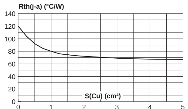
Fig. 8: Thermal resistance junction to ambient versus copper surface under each lead (Epoxy printed circuit board FR4, copper thickness:
