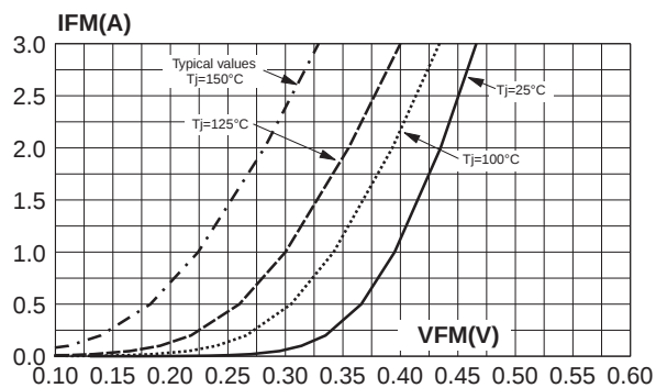
Fig. 7-3: Forward voltage drop versus forward current (maximum values, low level).
