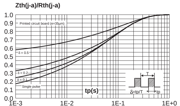
Fig. 4-3: Relative variation of thermal transient impedance junction to lead versus pulse duration (DPAK).
