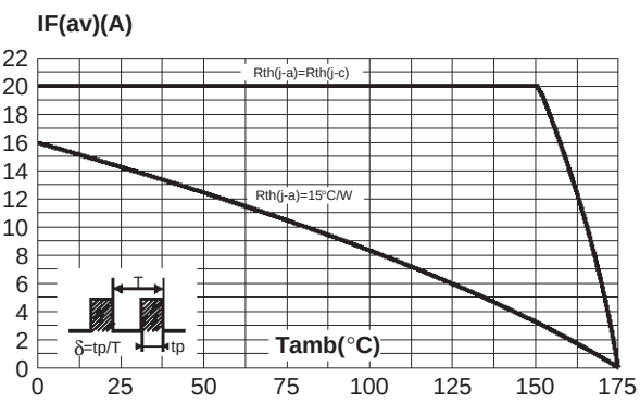
Fig. 2: Average current versus ambient temperature (per diode).
