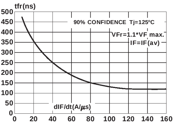
Fig. 9: Forward recovery time versus dI_F/dt .
