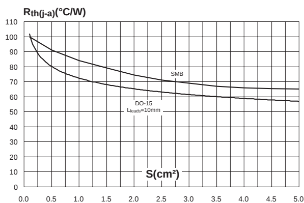
Fig. 4: Thermal resistance junction to ambient versus copper surface under each lead (epoxy printed circuit board FR4, copper thickness: 35μm).
