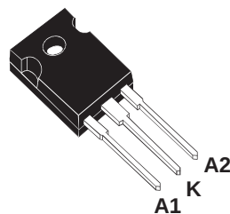
TO-247 STTH30R06CW
