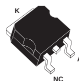
D²PAK STTH8R03G
