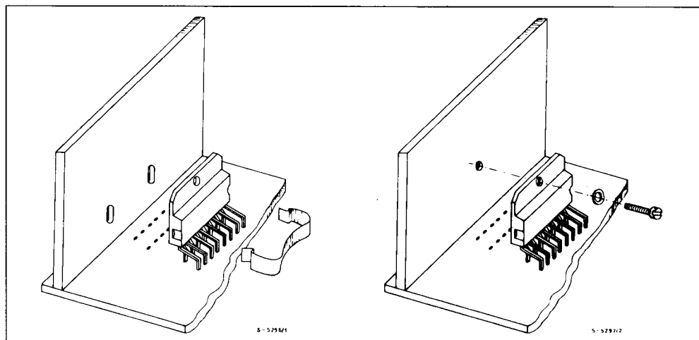
Figure 10 : Mounting Example.
